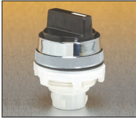
T11MA03-E maintained, three position, knob handle, black selector switch with clip and two contacts
