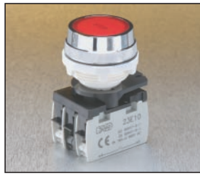
T11AJ10-CL24 momentary, round, flush, red pushbutton with clip, two contacts, lamp block and 24V LED bulb
